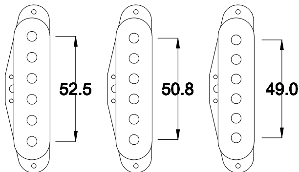
Maße ST TrueSpaceCovers
